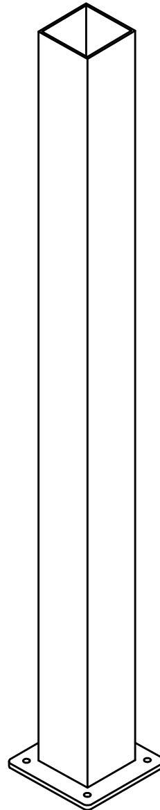
3"x .125" POST/ 5"x5" BASE PLATE
