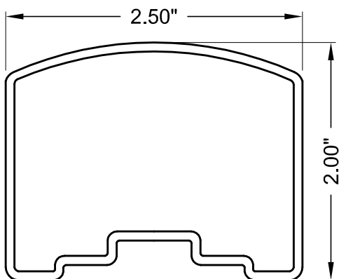
RECTANGULAR TOP PICKET
