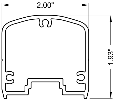
ORCA SQUARE TOP PICKET
